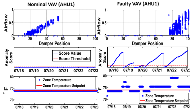
Figure 9. Comparisons between nominal (healthy) and faulty VAV units
