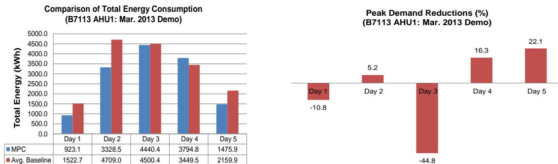
Figure 13. Total energy consumption and peak power reductions of MPC and baseline algorithms
