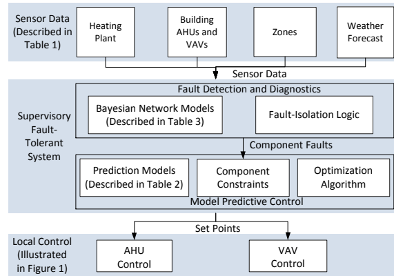
Figure 6. Hierarchical architecture of the fault-tolerant system
