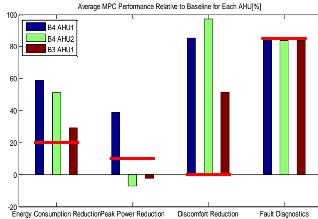
Figure 8. Illustration of the overall results generated during the demonstrations for MPC and FDD algorithms for each of the AHUs for the following objectives: energy consumption reduction, peak power reduction, thermal discomfort reduction, and fault diagnostics system robustness.
