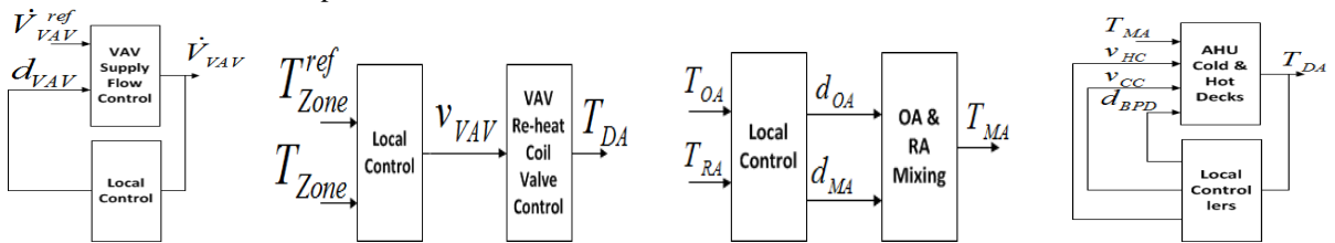
Figure 1. Signal flows of the VAV local control loops corresponding to supply air flow rate and zone temperature; Signal flows of the AHU local control loops corresponding to mixed air and discharge air temperatures
