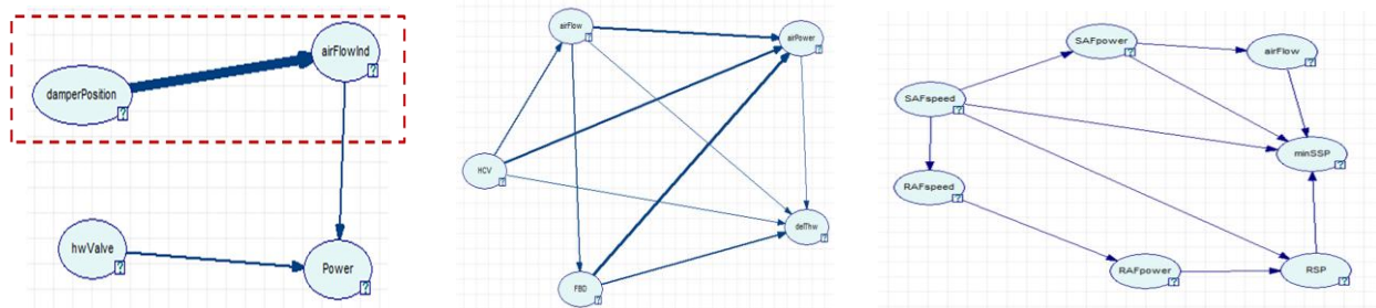
Figure 4. Graphical FDD models for the following actuators: outdoor air damper (left); AHU heating coil (center); AHU fans (right)
