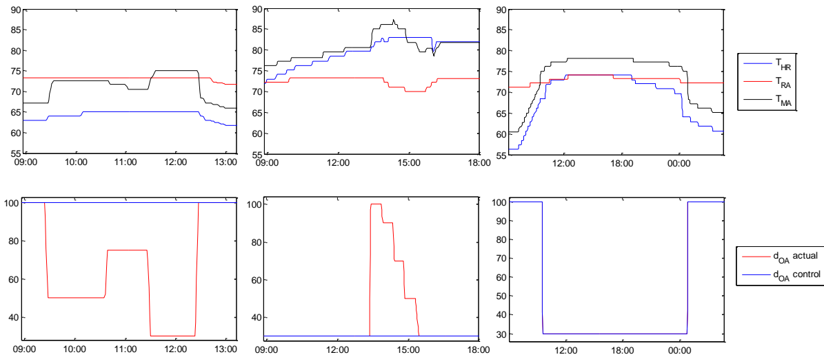
Figure 10. Illustration of the outdoor air damper positions and impacted temperatures for three scenarios described above the figure
