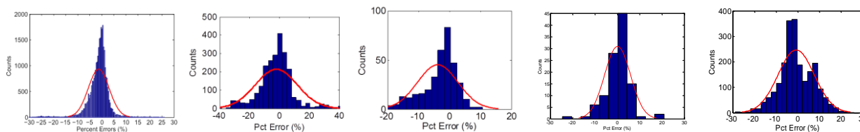
Figure 3. Histograms of the validation errors for all models of Table 2 (in the same order as in the table: mixed-air temperature; AHU heating coil thermal power; AHU supply air flow rate; AHU supply fan power; VAV re-heat coil thermal power)
