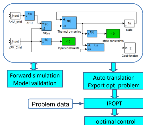
Figure 7. The main steps for converting the MPC algorithm into an optimization problem formulation using BLOM Table 4 presents typical performance of the BLOM library with IPOPT solver for the MPC problem formulated in Section 4.1. We present the execution time of problem solution for various problem sizes. The table shows that even
