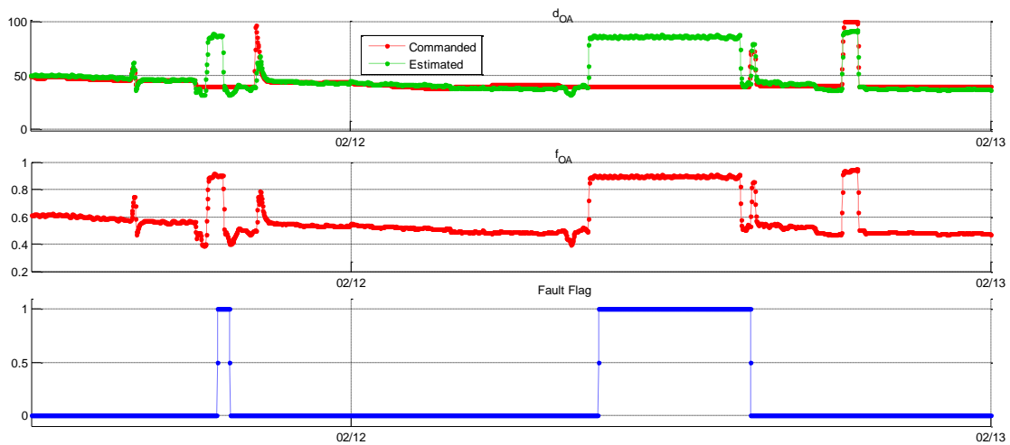
Figure 5. Illustration of validation test data for the FDD algorithm associated with outdoor air damper Outdoor air damper: BAS command, which was overridden; estimated position (top); outdoor air fraction (middle); fault flag (bottom)
