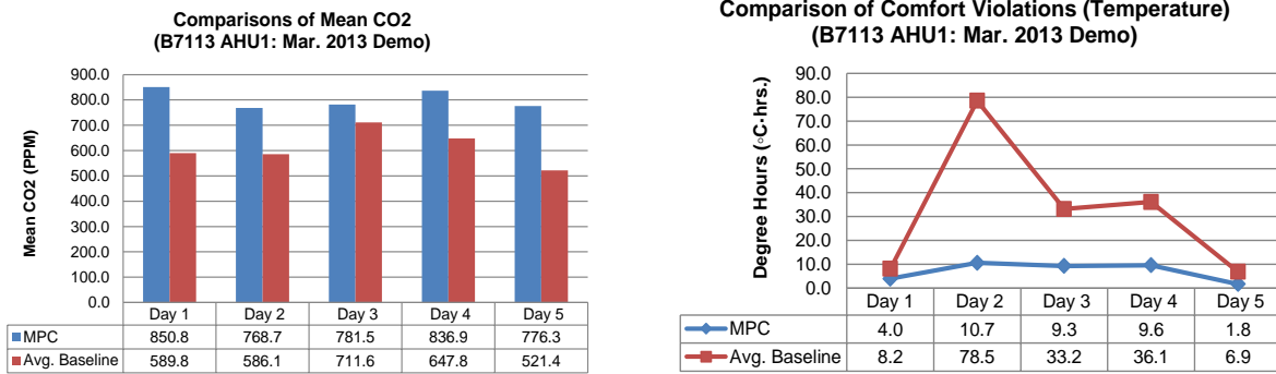
Figure 14. Mean zone CO 2 levels and temperature comfort violation levels for MPC and baseline algorithms
