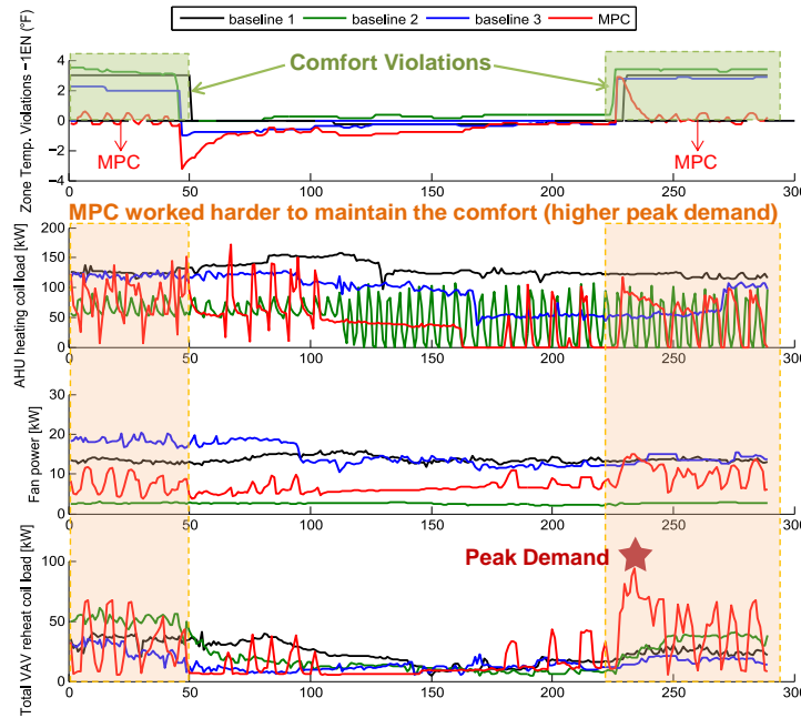
Figure 12. Illustration of temperature comfort violations, AHU heating coil power, fan power and total VAV thermal power during the same days as those illustrated in Figure 11.
