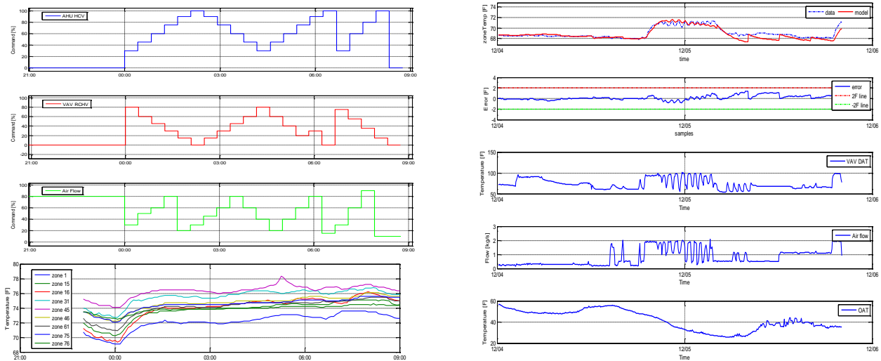
Figure 2. (Left) Normalized time series data of the inputs v_{AHU,HC} , v_{VAV_i,HC} , and \dot{m}_{sa,S_i} for a system identification test for AHU 1 , and corresponding zone temperatures measurements; (Right) Model validation results using new data sets based on which it was concluded that the zone temperature modeling error is smaller than 2 0 F
